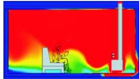
Heat distribution with an Ecofan ®
